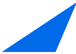
Scalene triangle
